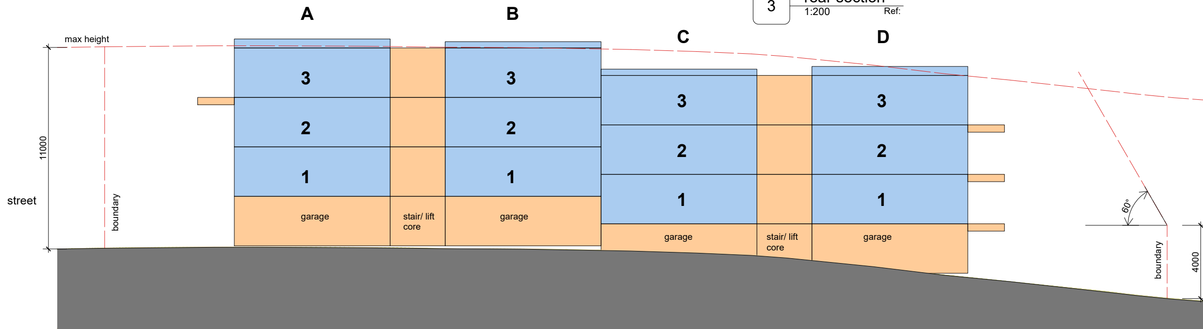
4 long section 1:200 Ref:
