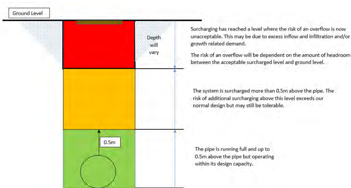
Figure 3.1.2 Colour Code for Dry and Wet Weather Pipe Condition
