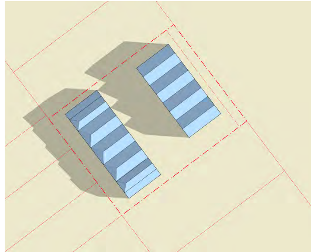
10 sun study Dec 20 9am 1:750 Ref:
