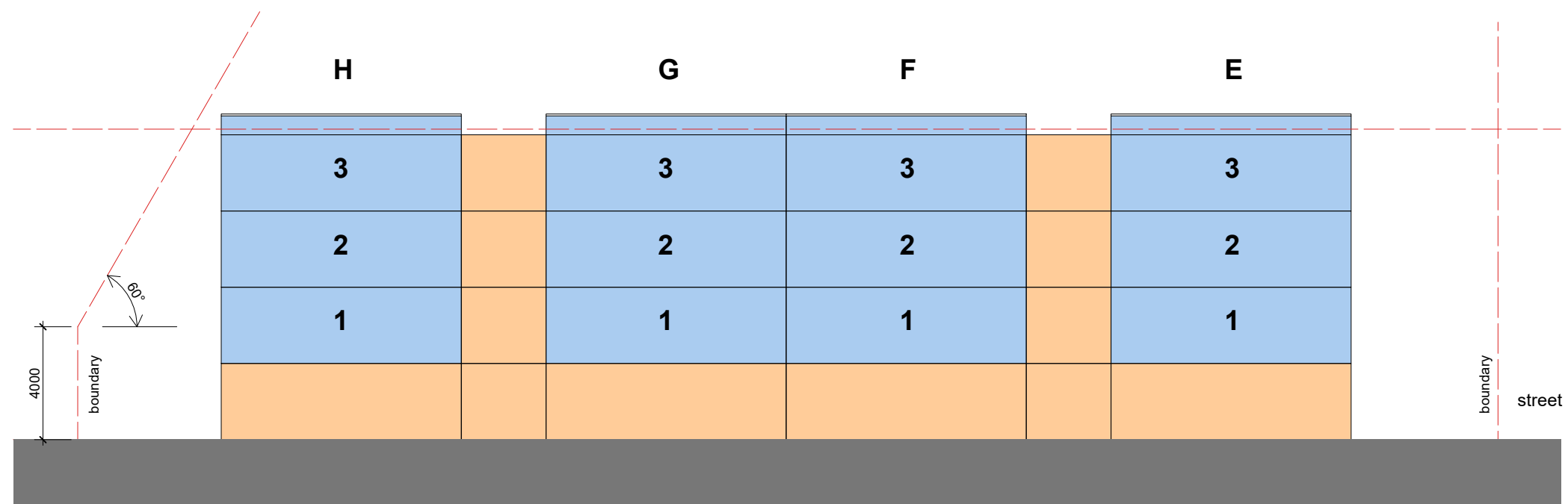
3 long section 1:200 Ref:
